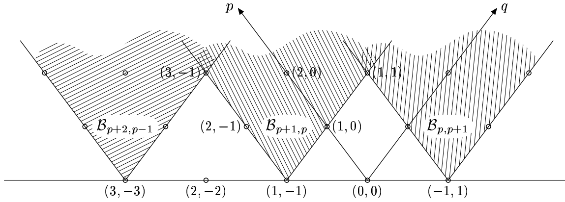
FIGURE 2. The augmentation bigrading on \mathcal{B}_{k+1}^\bullet for an even k , k = 2p .
