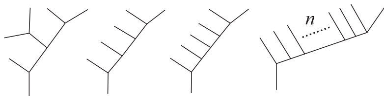
Figure 12: From left to right, the non-simple tree of lowest-order (order-4) and the simple trees of order 4, 5 and 6 + n .
