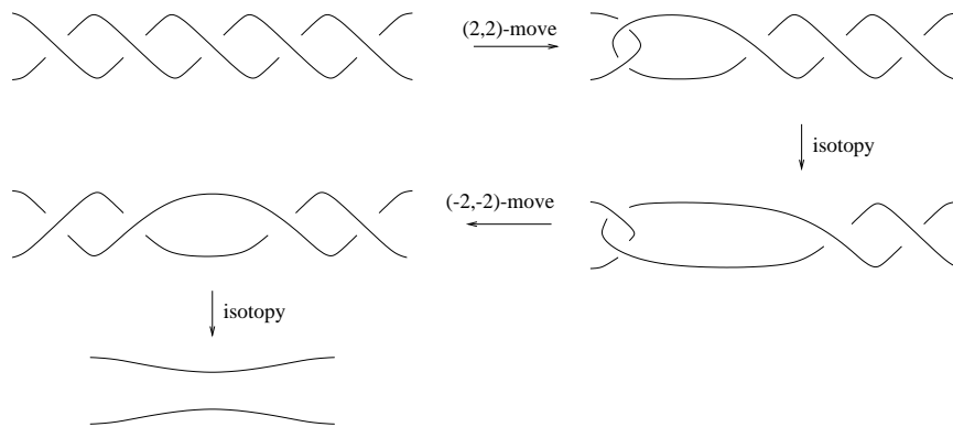
Figure 1.7: 5-move as a combination of \pm(2, 2) -moves
