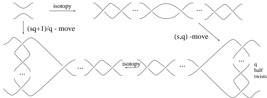
Figure 1.12: (s, q) -move as \frac{sq+1}{q} -move
