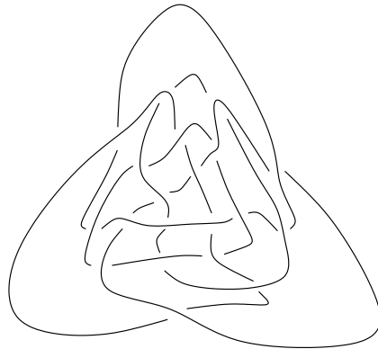
Figure 1.6: L_{2BR} and the Chen's link
