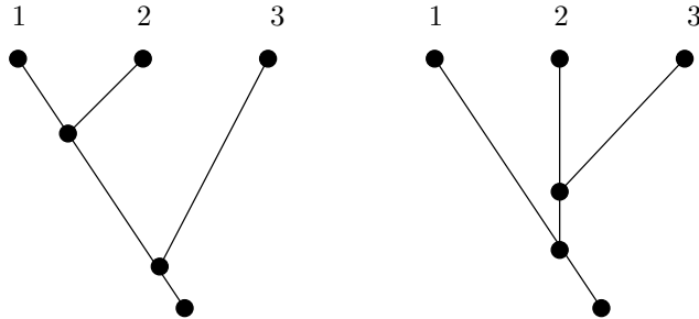
Figure 5: Constructing planar weighted trees
