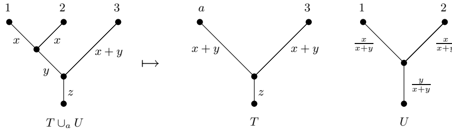
Figure 9: The map \overline{w}(T \cup_a U) \rightarrow \overline{w}(T) \wedge \overline{w}(U)
