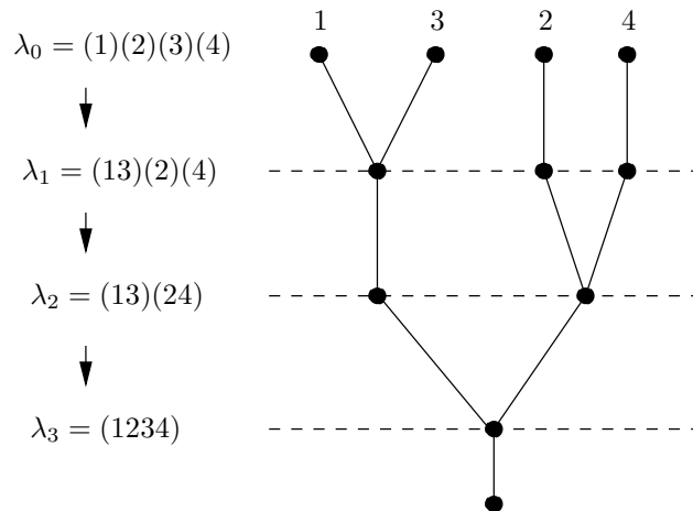
Figure 7: Producing trees from sequences of partitions
