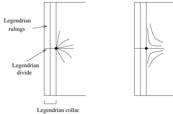
Figure 5: Equivalences in the shufflable case
