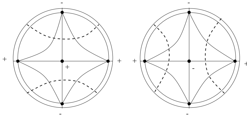
Figure 2: Inductive step
