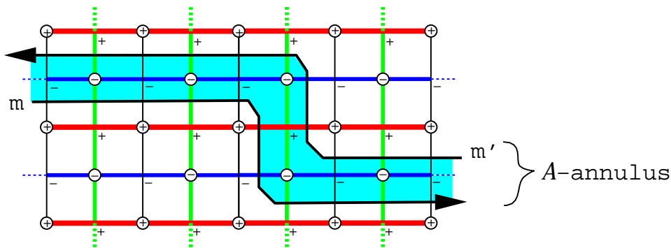
Figure 13: The shaded region between m and m' is \mathcal{A} . Notice that the induced foliation of \mathcal{A} has only aa -singularities.
