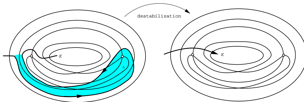
Figure 9: K enters into the foliated region and intersects a singular leaf twice. This allows for a destabilization of K . The shaded region \Delta corresponds to the \Delta of Lemma 2.5.
