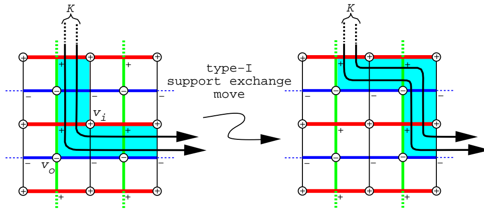
Figure 11: The alteration in \mathcal{S}_K from left to right corresponds to an exchange move with type-I support. The vertex labeled v_o is an outside vertex and the vertex labeled v_i is an inside vertex. The shaded region is a portion of \mathcal{S}_K .
