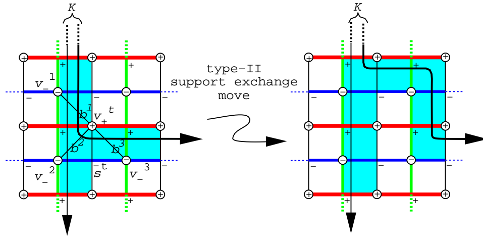
Figure 12: The alteration in \mathcal{S}_K from left to right corresponds to an exchange move with type-II support. The vertex labeled v_\epsilon^t is a tee vertex and the singularity labeled s^t is a tee singularity. The shaded region indicates a portion of \mathcal{S}_K .
