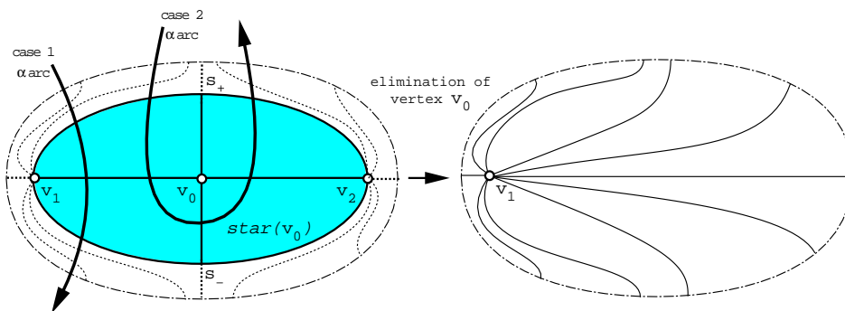
Figure 6: The vertex v_0 is a type (b,b) vertex. In the situation where the case 2 \alpha arcs are absent, after an exchange move, the \mathbf{b} -arcs between v_0 and v_2 are inessential.
