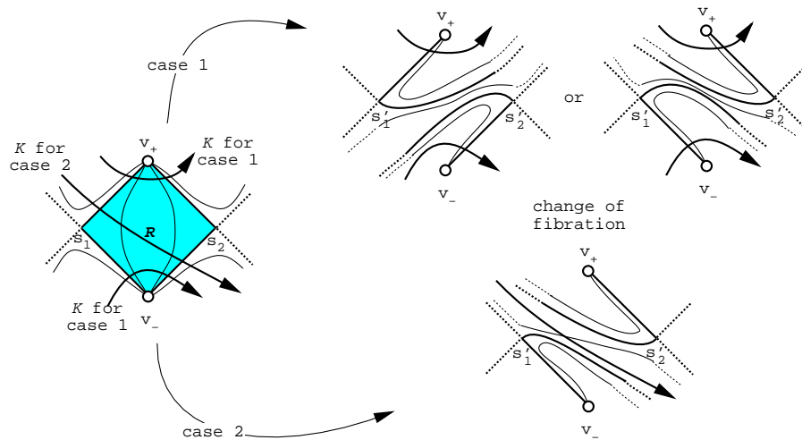
Figure 5: Parity of s_1 equals parity of s_2 . In case 1 there are two possible ways to change the fibration of \mathbf{H} and, thus, the foliation of \mathcal{T}_C . In case 2 there is only one way to alter the fibration.
