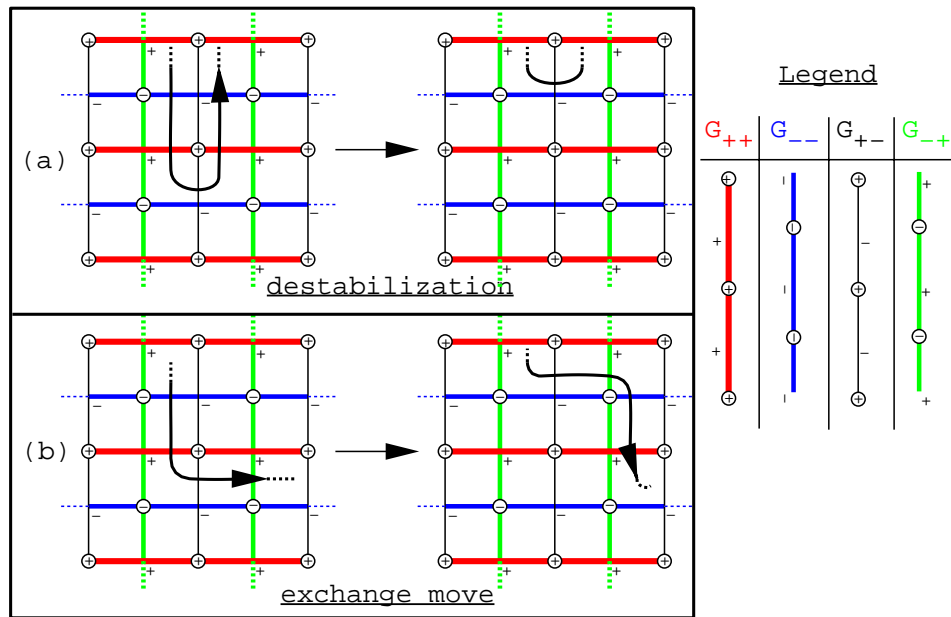
Figure 10: In (a) the intersection pattern is G_{-,-} \rightarrow G_{+,+} \rightarrow G_{-,+} \rightarrow G_{+,+} \rightarrow G_{-,-} . In (b), the intersection pattern is G_{-,-} \rightarrow G_{+,+} \rightarrow G_{+,-} \rightarrow G_{-,+} .
