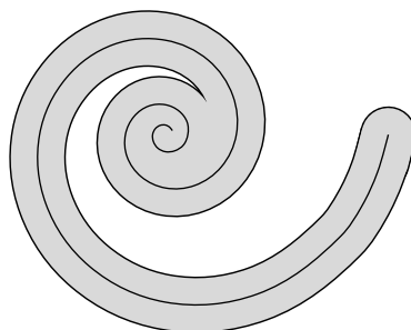
Figure 2: A self-nesting spiral-like body
