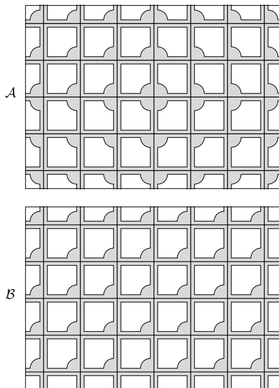
Figure 4: Packing a square with a mass in one corner
