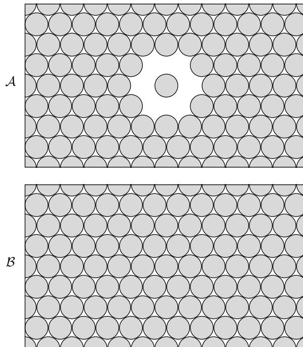
Figure 1: Two dense circle packings
