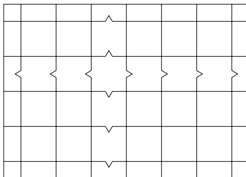
Figure 5: A solid tiling which is not weakly recurrent
