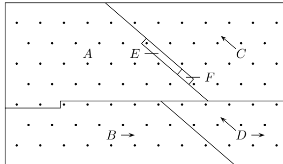
Figure 6: Tightening the hexagonal circle packing
