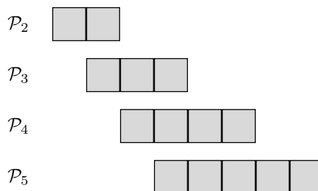
Figure 3: Anomalously replacing one square by two
