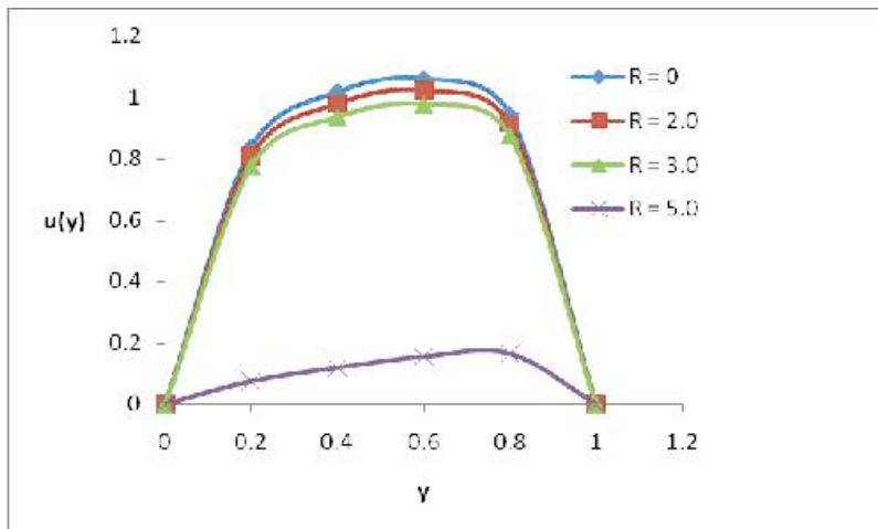
Figure 10: Dimensionless temperature profiles against y at Na_0 = 100
