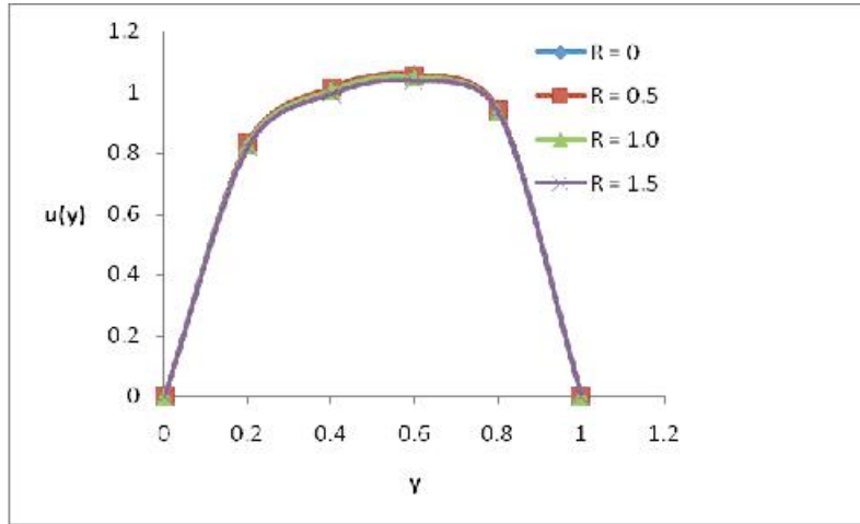
Figure 9: Dimensionless temperature profiles against y at Na_0 = 100
