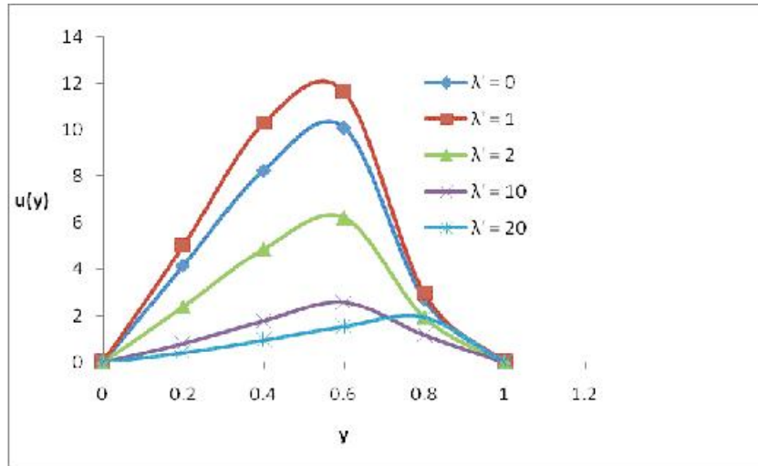
Figure 5: Dimensionless velocity profiles against y at M = 2
