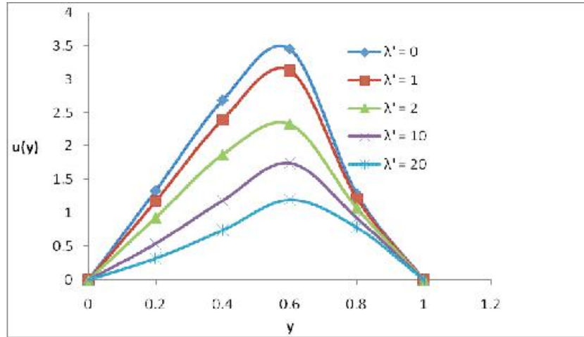
Figure 3: Dimensionless velocity profiles against y at M = 1
