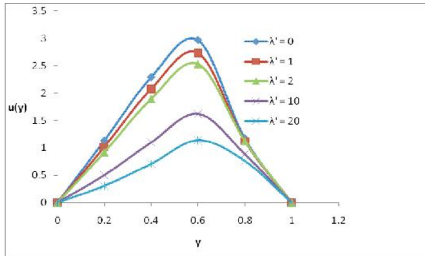
Figure 2: Dimensionless velocity profiles against y at M = 0.5
