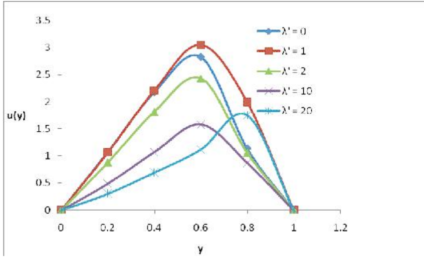
Figure 1: Dimensionless velocity profiles against y at M = 0
