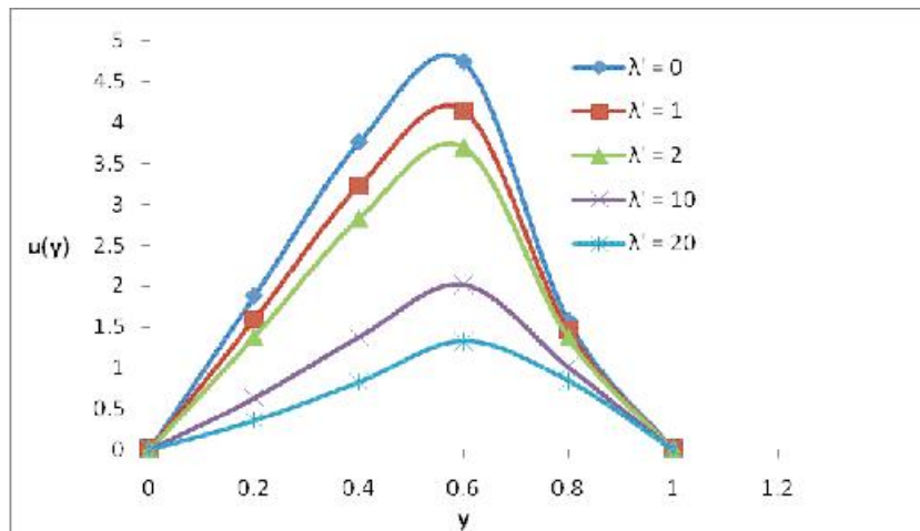
Figure 4: Dimensionless velocity profiles against y at M = 1.5
