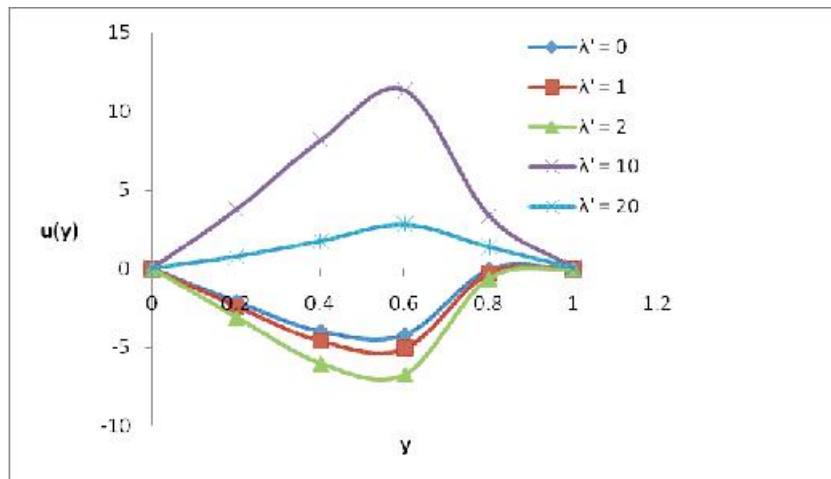
Figure 6: Dimensionless velocity profiles against y at M = 3
