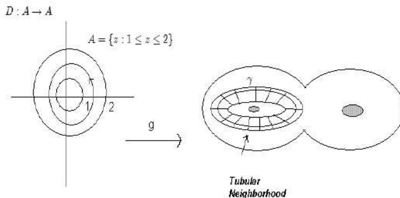
FIGURE 4. A right-handed Dehn twist on an oriented surface.
