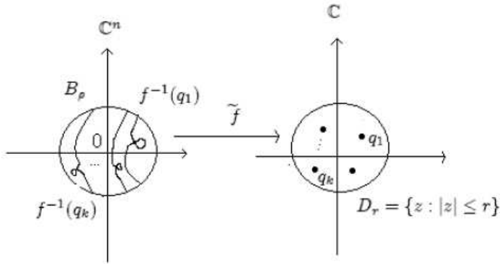
FIGURE 2. The structure of \tilde{f} .
