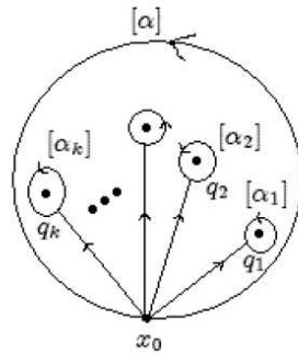
FIGURE 6. The system of curves \alpha_1, \dots, \alpha_k on the disk.
