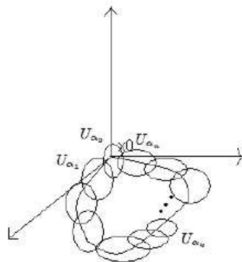
FIGURE 3. Trivialization of the bundle along \gamma .
