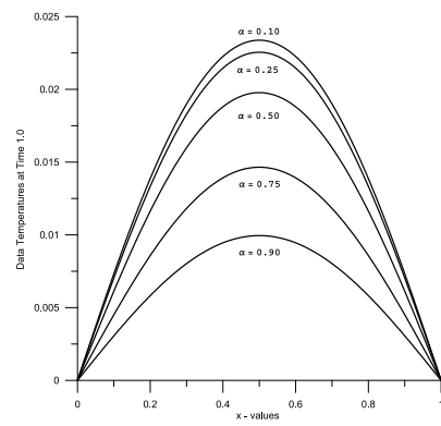
FIGURE 5. Exact Temperatures.
