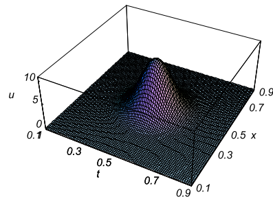
FIGURE 6. \alpha = 0.75 , \epsilon = 0.05 .
