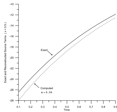
FIGURE 14. \alpha = 0.5, \epsilon = 0.05 .
