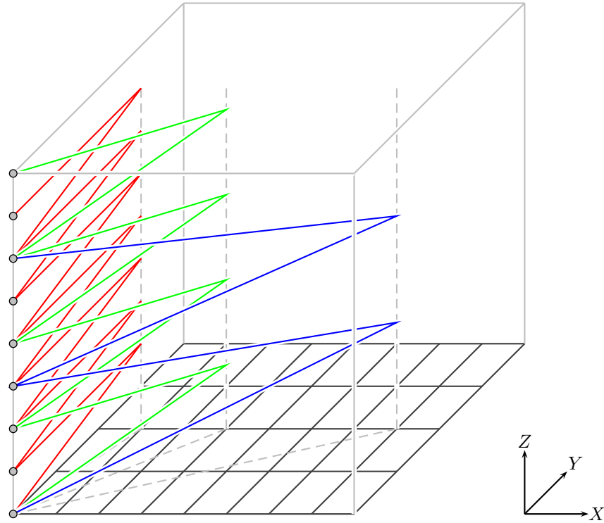
Figure 1: Construction of collinear 1-bend drawing in Lemma 3.
