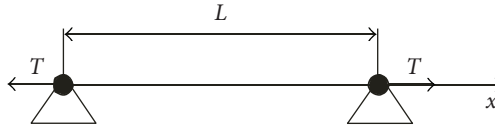
Figure 2.1. Conveyor belt model.
