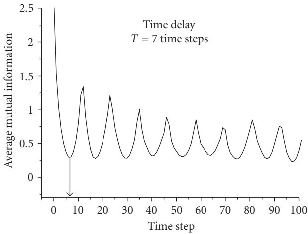
Figure 4.3. Average mutual information for the attractor 4. The first minimum corresponds to the optimal time delay.
