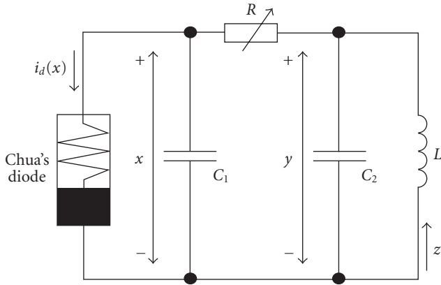
Figure 1.1. Chua's circuit. The dynamical variables are x , y , and z corresponding to the voltage across capacitor C_1 , the voltage across capacitor C_2 , and the current through the inductor, respectively. The nonlinear element is the Chua's diode and the nonlinearity is presented through i_d(x) characteristics.
