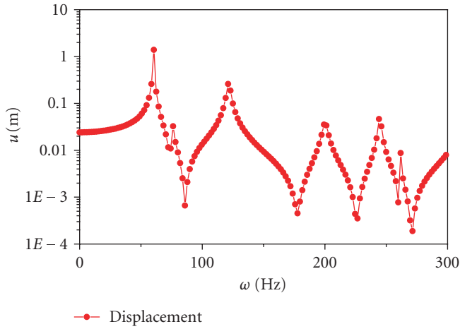
Figure 5.4. FRF_{18-18} for the first BE discretization of the two SFBS plates.
