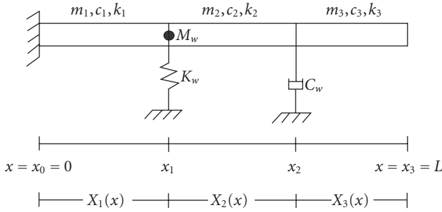
Figure 2.1. A triple-span discontinuous cantilever beam.
