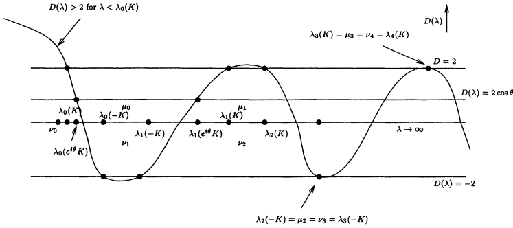
FIGURE 1 The graph illustrating the inequalities in (3.9) is the same except that \nu_n moves to the position of \nu_{n+1} for all n \in \mathbb{N}_0 .
