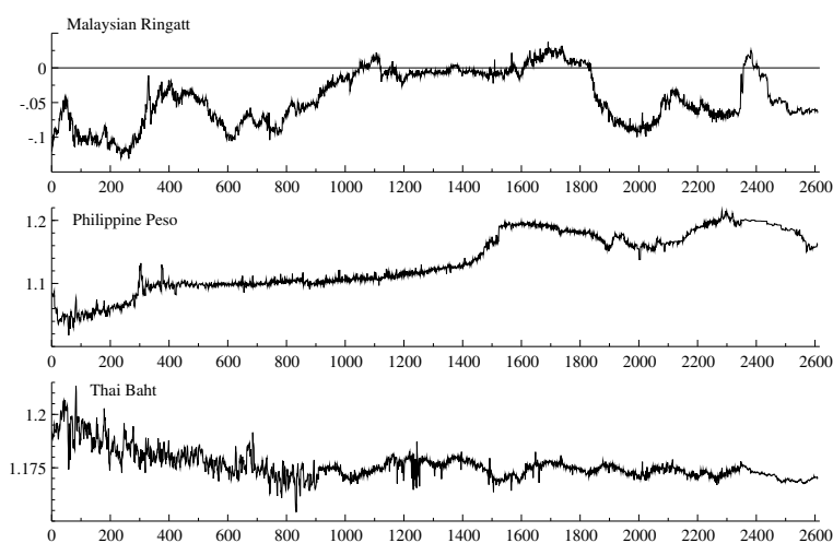
Figure 4. Time series plots of the natural logarithms of the Malaysian Ringgit, Philippine Peso and Thai Baht exchange rates respectively.
