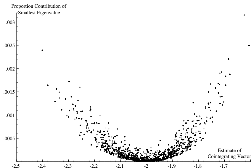
Figure 1. Cross-plot of the estimate of the cointegrating vector via the RBC procedure and the proportion contribution of the smallest eigenvalue for 10000 simulations of Example 1.
