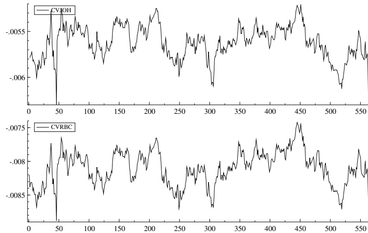
Figure 3. Time series plots of the linear combinations of the cointegrating vector via the Johansen Method and RBC procedure respectively for the spot and forward data.
