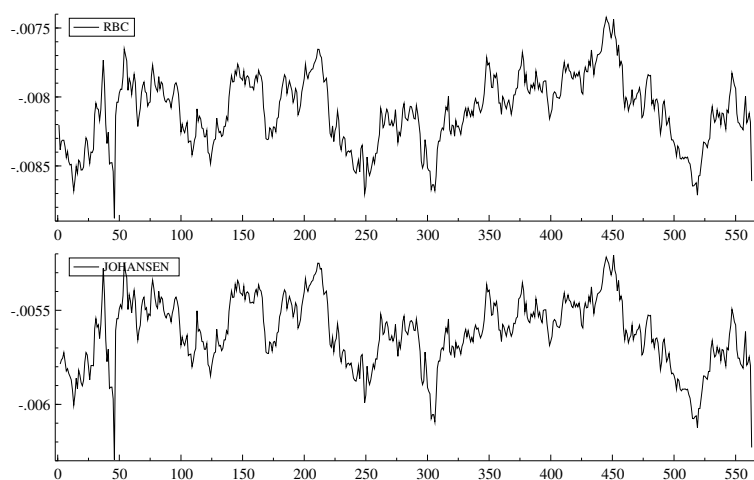
Figure 5. Time series plots of the linear combinations of the RBC and Johansen cointegrating vectors respectively for the Asian exchange rate data.
