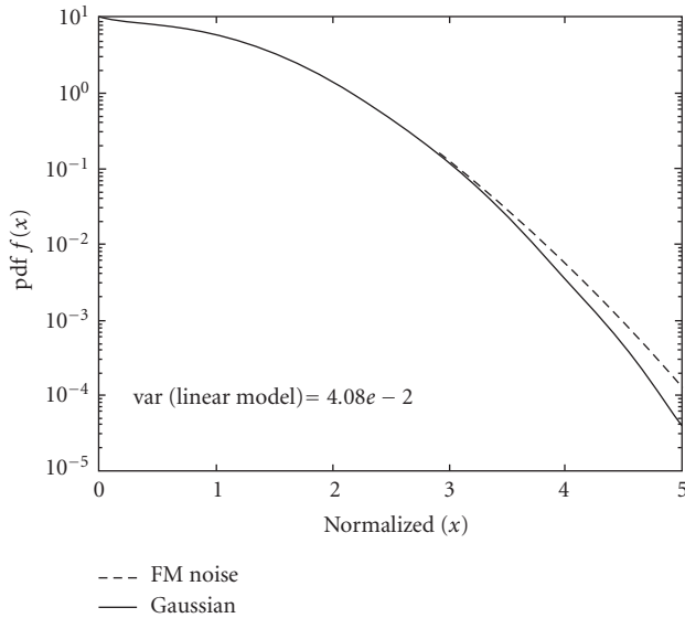
Figure 3.2. FM demodulator output noise pdf (SNR = 20 dB).
