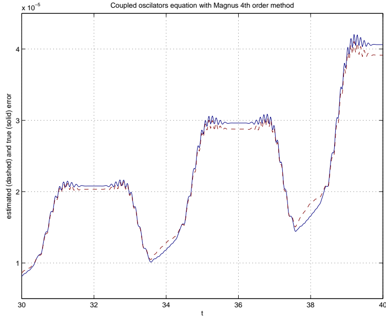
FIG. 6.3. True (solid) and estimated (dashed) errors for the coupled oscillator equation (6.2), computed by a fourth order Magnus method with step-size h = 2^{-6} on [0, 40] . Only the interval [30, 40] is shown.
