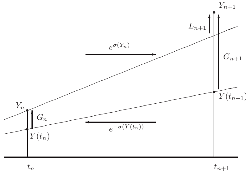
FIG. 3.1. The relation between the global errors at t_n and at t_{n+1} and the local error at t_{n+1} (A slice of the Lady Windermere's fan [9]).
