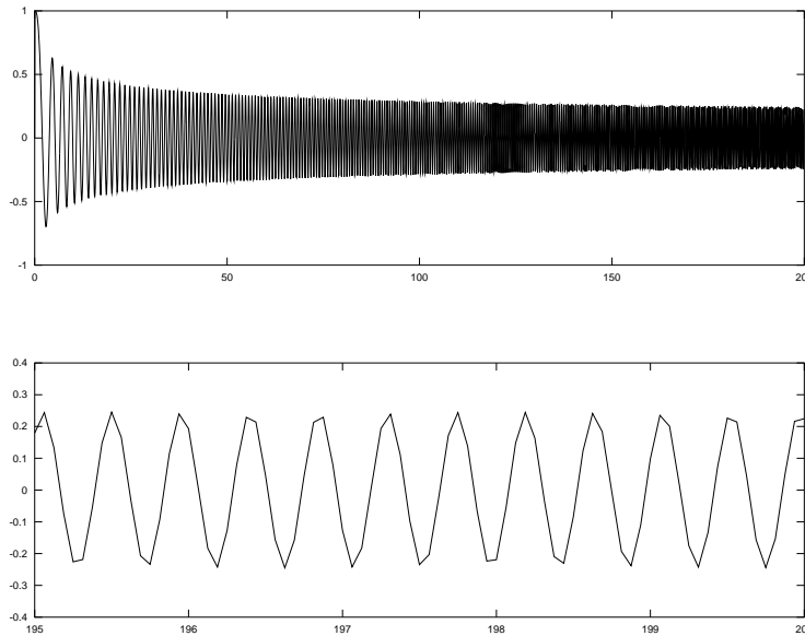
FIG. 6.1. The numerical solution of the Airy equation (6.1) on the whole interval [0, 200] (above) and on interval [195, 200] (below).
