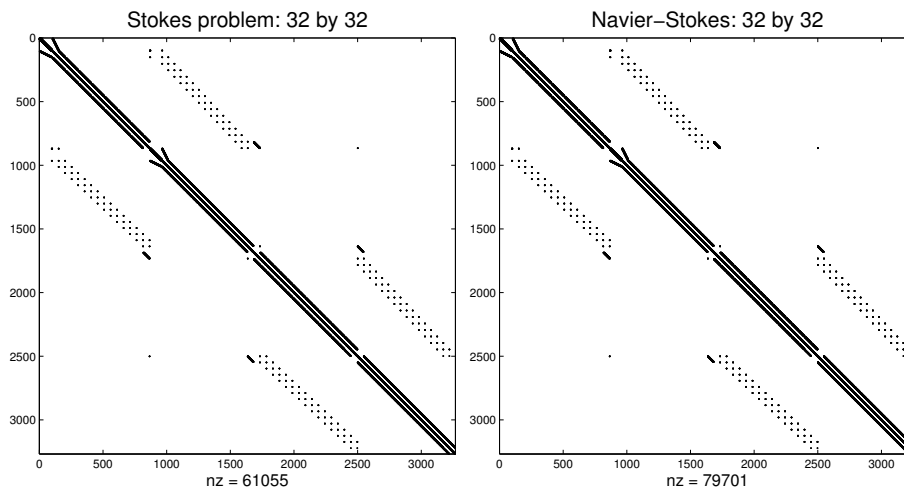
FIG. 2.1. Nonzero pattern of the discrete Stokes matrix (left) and the Jacobian matrix (right) for Re = 1,000 on a 32 \times 32 mesh. nz is the number of nonzero elements.
