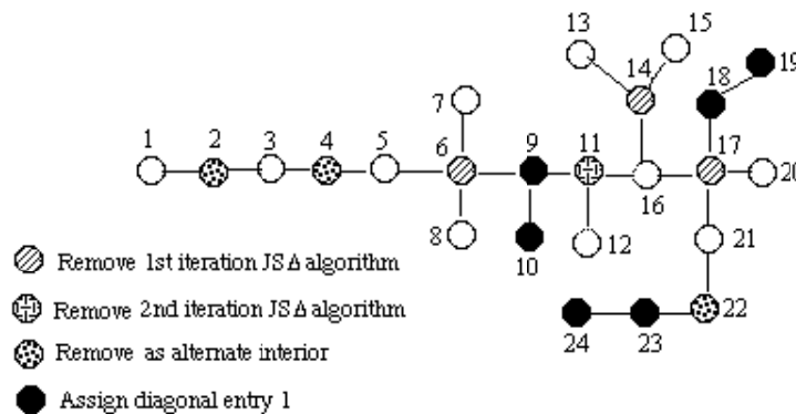
FIG. 4.1. Applying Algorithm 4.3 to a tree T .
