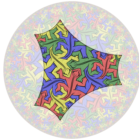
(b) Colored fundamental domain
