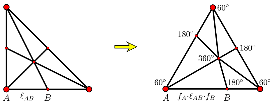
Figure 9: Example of conformal equivalence
