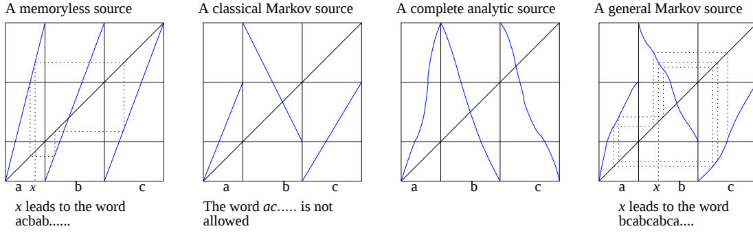
Fig. 4: Memoryless and classical Markov sources
