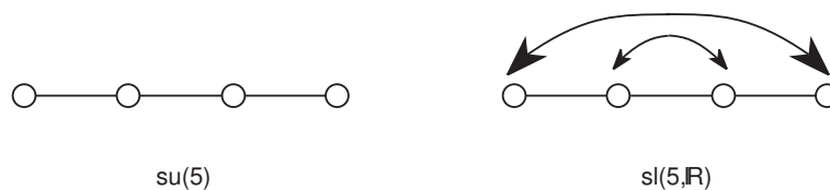
Figure 32: The Vogan diagrams for \mathfrak{su}(5) and \mathfrak{sl}(5, \mathbb{R}) .
