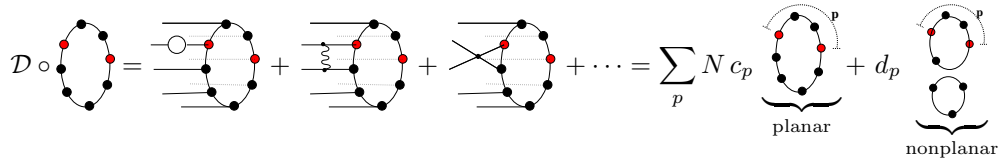
Figure 4: The action of the dilatation operator on a trace operator.
