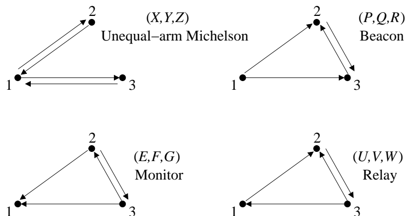
Figure 5: Schematic diagrams of the unequal-arm Michelson, Monitor, Beacon, and Relay combinations. These TDI combinations rely only on four of the six one-way Doppler measurements, as illustrated here.
