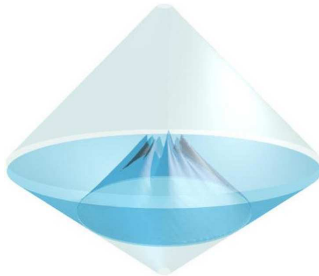
Figure 7: The geometry of the asymptotic characteristic initial value problem: Characteristic data are given on the blue parts, i.e. an ingoing null surface and the part of \mathcal{I}^- that is in its future. Note that the ingoing surface may develop self-intersections and caustics.
