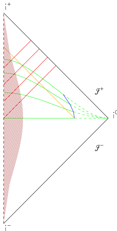
Figure 9: The geometry of the standard Cauchy approach. The green lines are surfaces of constant time. The blue line indicates the outer boundary.
