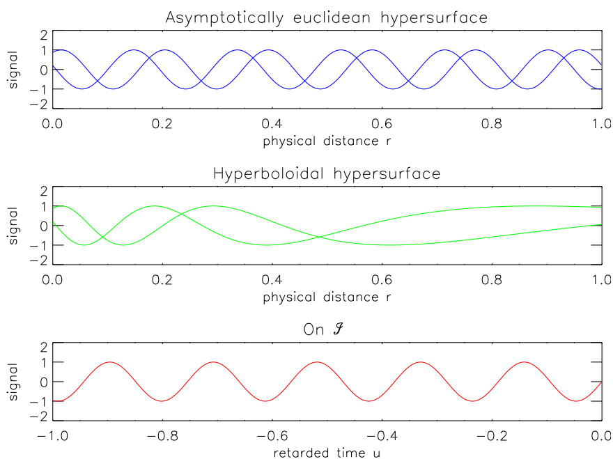
Figure 4: Waveforms in physical space-time.
