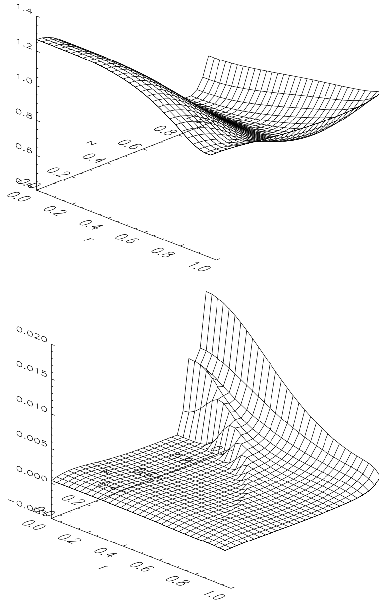
Figure 12: An axi-symmetric solution of the Yamabe equation with u = 1 on the boundary (top) and its third differences in the z -direction (bottom). The location of \mathcal{S} is clearly visible.
