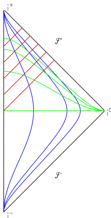
Figure 2: The conformal diagram of Minkowski space.
