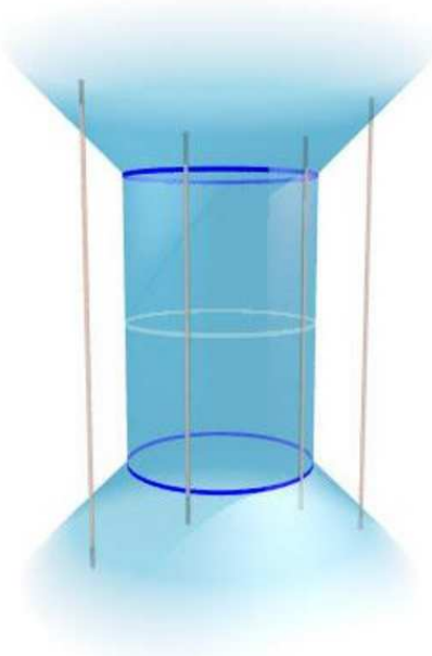
Figure 8: The geometry near space-like infinity: The “point” i^0 has been blown up to a cylinder that is attached to \mathcal{S}^- and \mathcal{S}^+ . The physical space-time is the exterior part of this “stovepipe”. The “spheres” I^\pm and I^0 are shown in blue and light green, respectively. The brown struts symbolize the conformal geodesics used to set up the construction. Note that they intersect \mathcal{S} and continue into the unphysical part.
