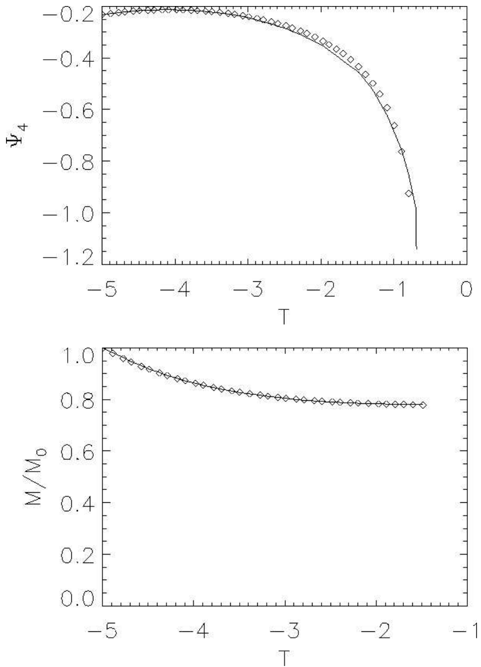
Figure 16: The radiation field \psi_4 and the Bondi mass for a radiating A3-like space-time.
