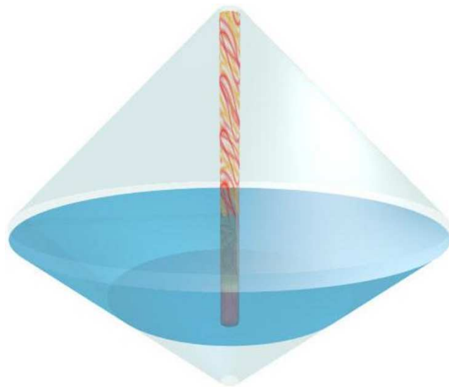
Figure 6: The physical scenario: The figure describes the geometry of an isolated system. Initial data are prescribed on the blue parts, i.e. on a hyperboloidal hypersurface and the part of \mathcal{I}^- which is in its future. Note that the two cones \mathcal{I}^+ and \mathcal{I}^- are separated to indicate the non-trivial transition between them.
