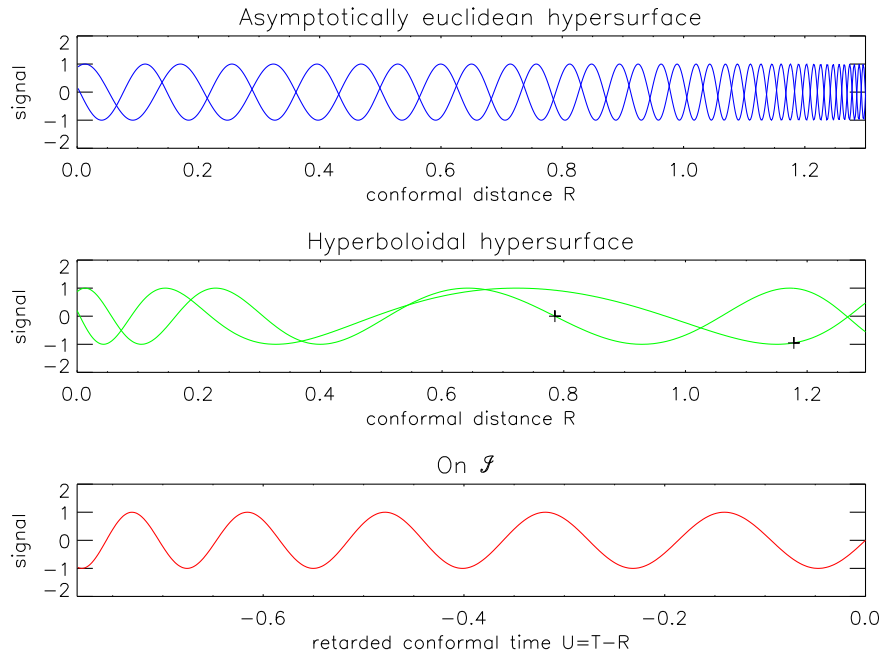
Figure 5: Waveforms in conformal space-time.
