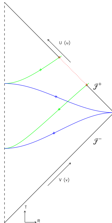
Figure 3: Spacelike hypersurfaces in the conformal picture.
