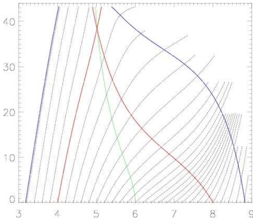
Figure 17: The numerically generated ‘Kruskal diagram’ for the Schwarzschild solution.
