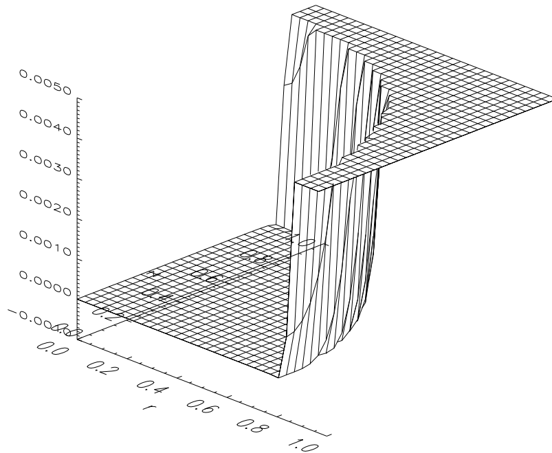
Figure 13: The difference between two solutions of the Yamabe equation obtained with different boundary conditions outside. Only the values less than 0.005 are shown.
