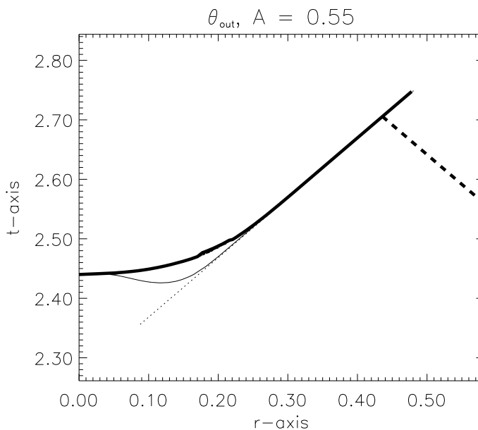
Figure 14: Upper corner of a space-time with singularity (thick line). The dashed line is \mathcal{I} , while the thin line is the locus of vanishing divergence of outgoing light rays, i.e. an apparent horizon.
