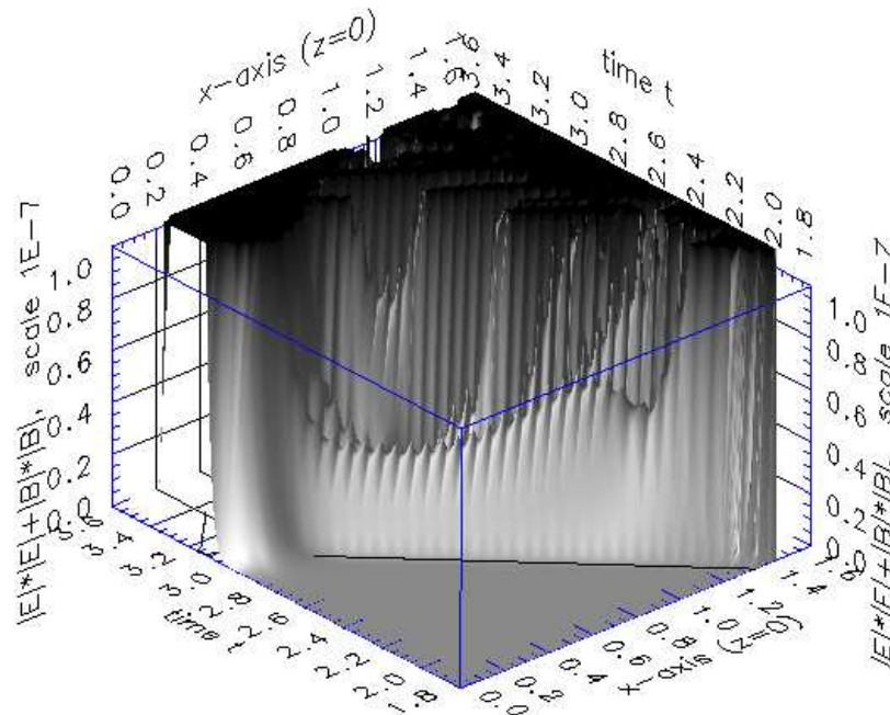
Figure 18: The rescaled Weyl tensor in a flat space-time obtained from flat initial data and random boundary data in the unphysical region.
