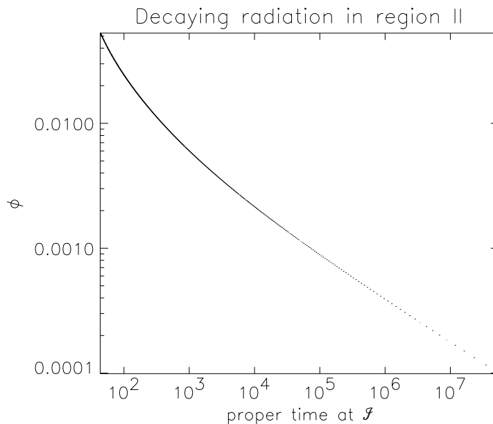
Figure 15: Decay of the radiation at null-infinity.
