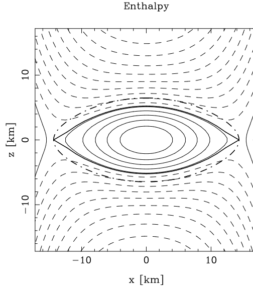
Figure 3: Meridional plane cross section of a rapidly rotating strange star at the mass-shedding limit, obtained with a multi-domain spectral code. The various lines are isocontours of the log-enthalpy H , as defined in [133]. Solid lines indicate a positive value of H and dashed lines a negative value (vacuum). The thick solid line denotes the stellar surface. The thick dot-dashed line denotes the boundary between the two computational domains. (Figure 4 of Gourgoulhon, Haensel, Livine, Paluch, Bonazzola, and Marck [133]; used with permission.)
