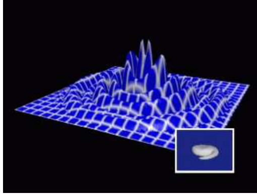
Figure 17: Still from a movie showing the gravitational wave emission during the development of the dynamical bar-mode instability in a rapidly rotating relativistic star. The gravitational wave amplitude in a plane containing the rotation axis is shown. At large distances, the waves assume a quadrupole-like angular dependence. Movie produced at the University of Illinois by T.W. Baumgarte, S.L. Shapiro, and M. Shibata, with the assistance of the Illinois Undergraduate Research Team [29]; used with permission. (To see the movie, please go to the electronic version of this review article at http://www.livingreviews.org/lrr-2003-3/ .)
