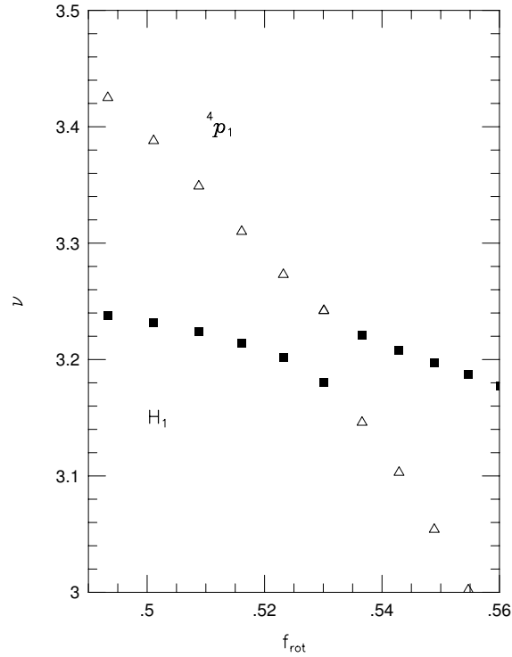
Figure 4: Apparent intersection (due to avoided crossing) of the axisymmetric first quasi-radial overtone ( H_1 ) and the first overtone of the l = 4 p-mode (in the Cowling approximation). Frequencies are normalized by \sqrt{\rho_c/4\pi} , where \rho_c is the central energy density of the star. The rotational frequency f_{\text{rot}} at the mass-shedding limit is 0.597 (in the above units). Along continuous sequences of computed frequencies, mode eigenfunctions are exchanged at the avoided crossing. Defining quasi-normal mode sequences by the shape of their eigenfunction, the H_1 sequence (filled boxes) appears to intersect with the {}^4p_1 sequence (triangle), but each sequence shows a discontinuity, when the region of apparent intersection is well resolved. (Figure 3 of Yoshida and Eriguchi [330]; used with permission.)
