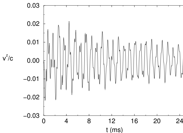
Figure 12: Evolution of the axial velocity in the equatorial plane for a relativistic r -mode in a rapidly rotating N = 1.0 polytrope (in the Cowling approximation). Since the initial data used to excite the mode are not exact, the evolution is a superposition of (mainly) the l = m = 2 r -mode and several inertial modes. The amplitude of the oscillation decreases due to numerical (finite-differencing) viscosity of the code. A beating between the l = m = 2 r -mode and another inertial mode can also be seen. (Figure 2 of Stergioulas and Font [294].)
