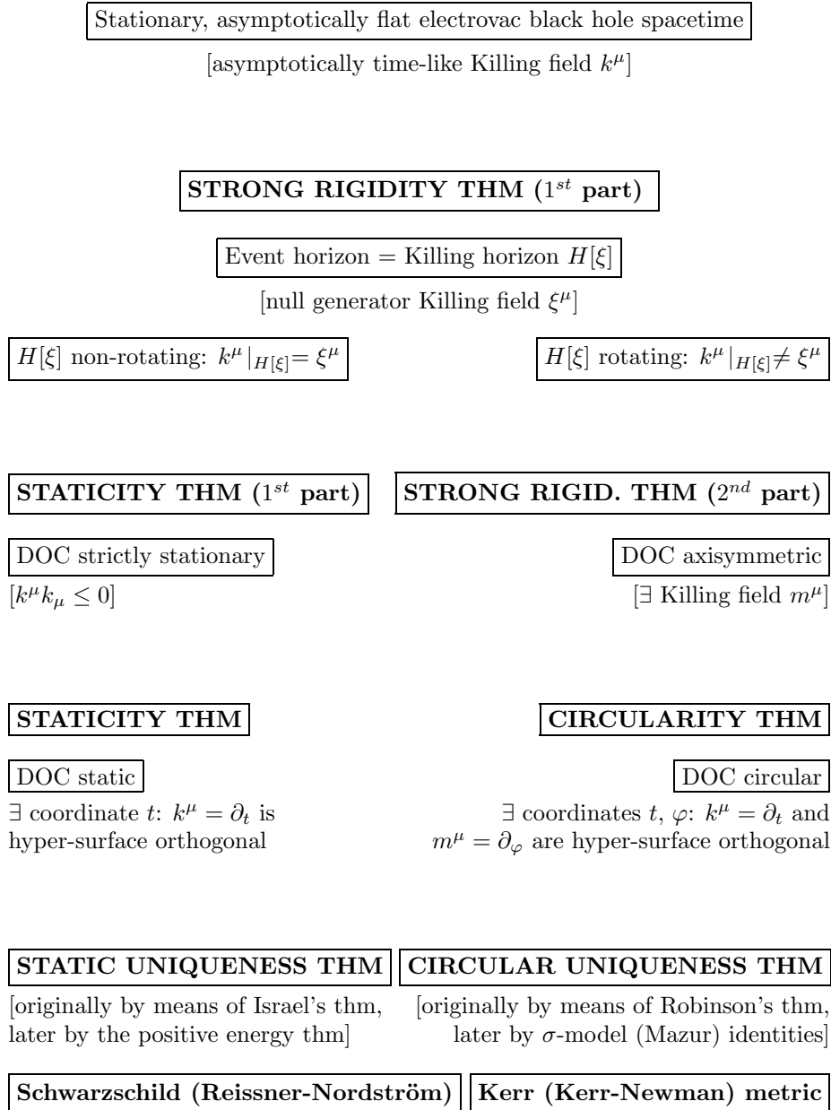
Figure 1: Classification of stationary electrovac black hole space-times
