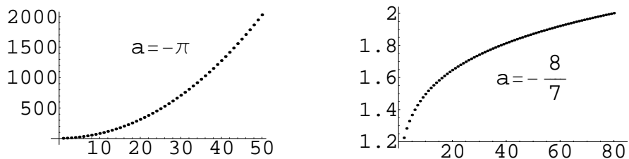
Figure 1: The sequences n \mapsto |C(a, n)| .
