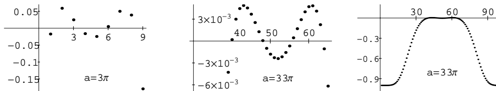
Figure 9: The graphs of sequences n \mapsto \rho(a, n) .
