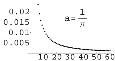
Figure 3: The sequences n \mapsto |C(a, n)| .
