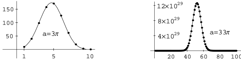
Figure 8: Approximations B(a, 2, x) to sequences n \mapsto C(a, n) .
