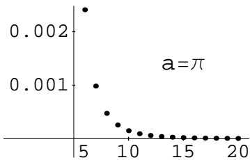
Figure 5: The sequences n \mapsto |C(a, n)| .
