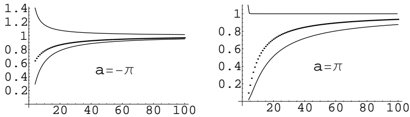
Figure 10: Estimating the sequence of binomial coefficients.
