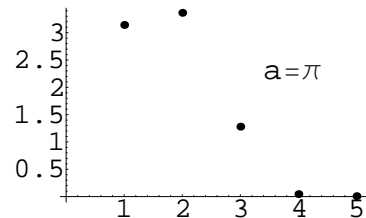
Figure 4: The sequences n \mapsto |C(a, n)| .
