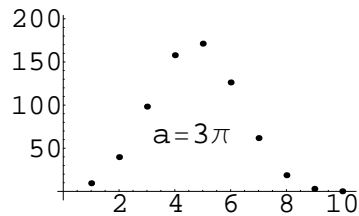
Figure 5: The sequences n \mapsto |C(a, n)| .
