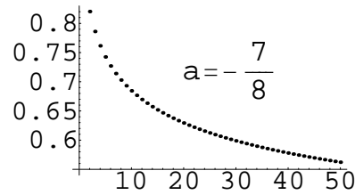
Figure 2: The sequences n \mapsto |C(a, n)| .
