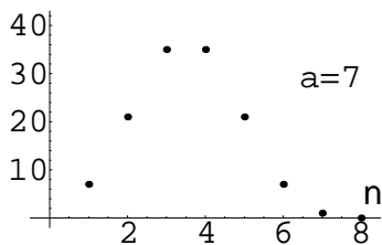
Figure 6: The sequences n \mapsto C(a, n) .
