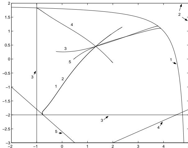
Figure 5: Repelling Paths of Example 3.1
