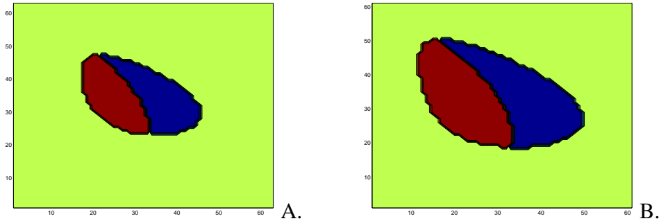
Figure 2: A) Slice of \mathcal{R} at height x_3 = 1 . B) Slice of \mathcal{R} at height x_3 = .9975
