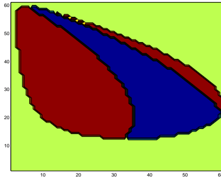
Figure 4: Slice of \mathcal{R} at height x_3 = .99
