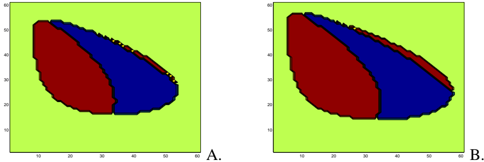
Figure 3: A) Slice of \mathcal{R} at height x_3 = .995 . B) Slice of \mathcal{R} at height x_3 = .9925
