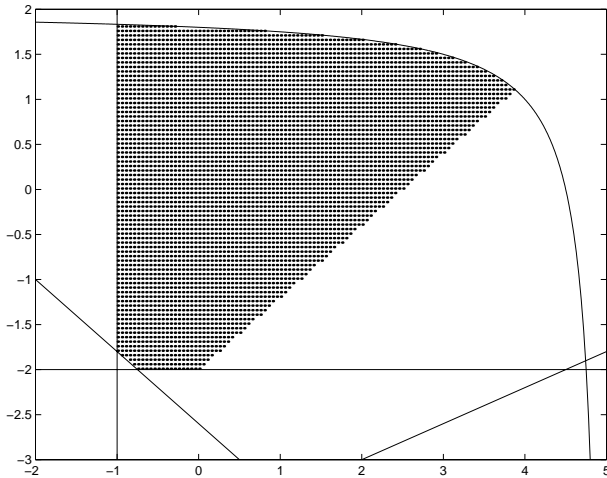
Figure 1: The region \mathcal{W} of weighted analytic centers bounded by the 5 constraints.
