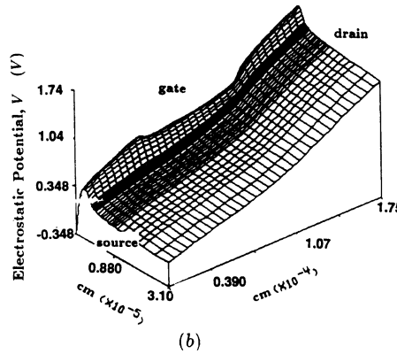
Figure 4. Electrostatic potential profiles for Device II with a gate voltage of 0.7 V and drain voltage of (a) 0.5 V, and (b) 1.35 V.
