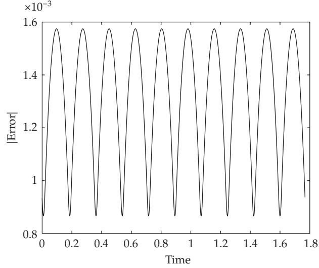
Figure 5: Behavior of the error in a sampling interval for LPWM scheme.
