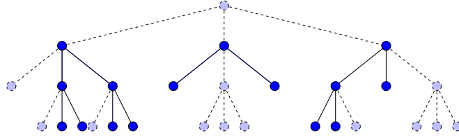
Figure 10: A ternary tree t and t^{deg} . Plain vertices belong to t^{deg} .
